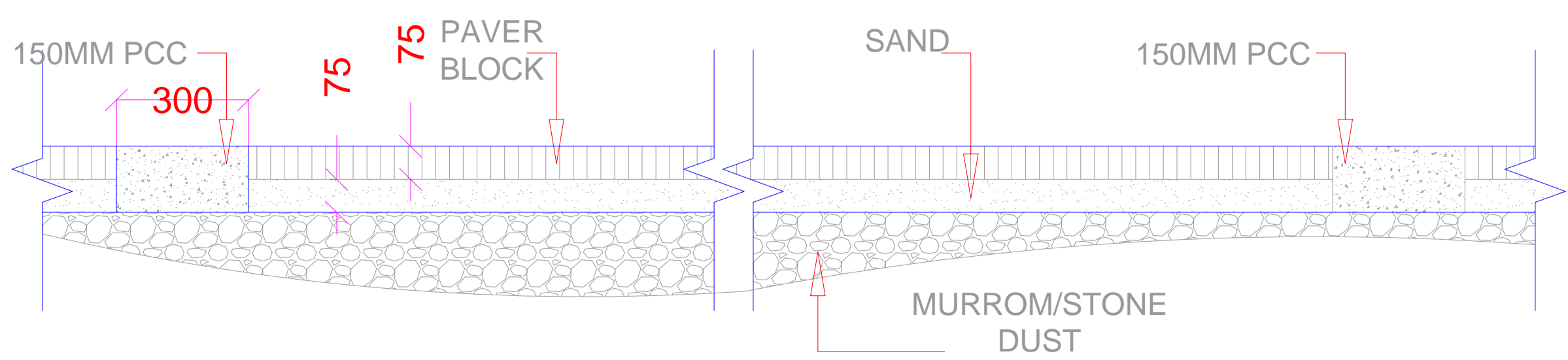
TYPICAL SECTION OF GROUND AT PARKING
